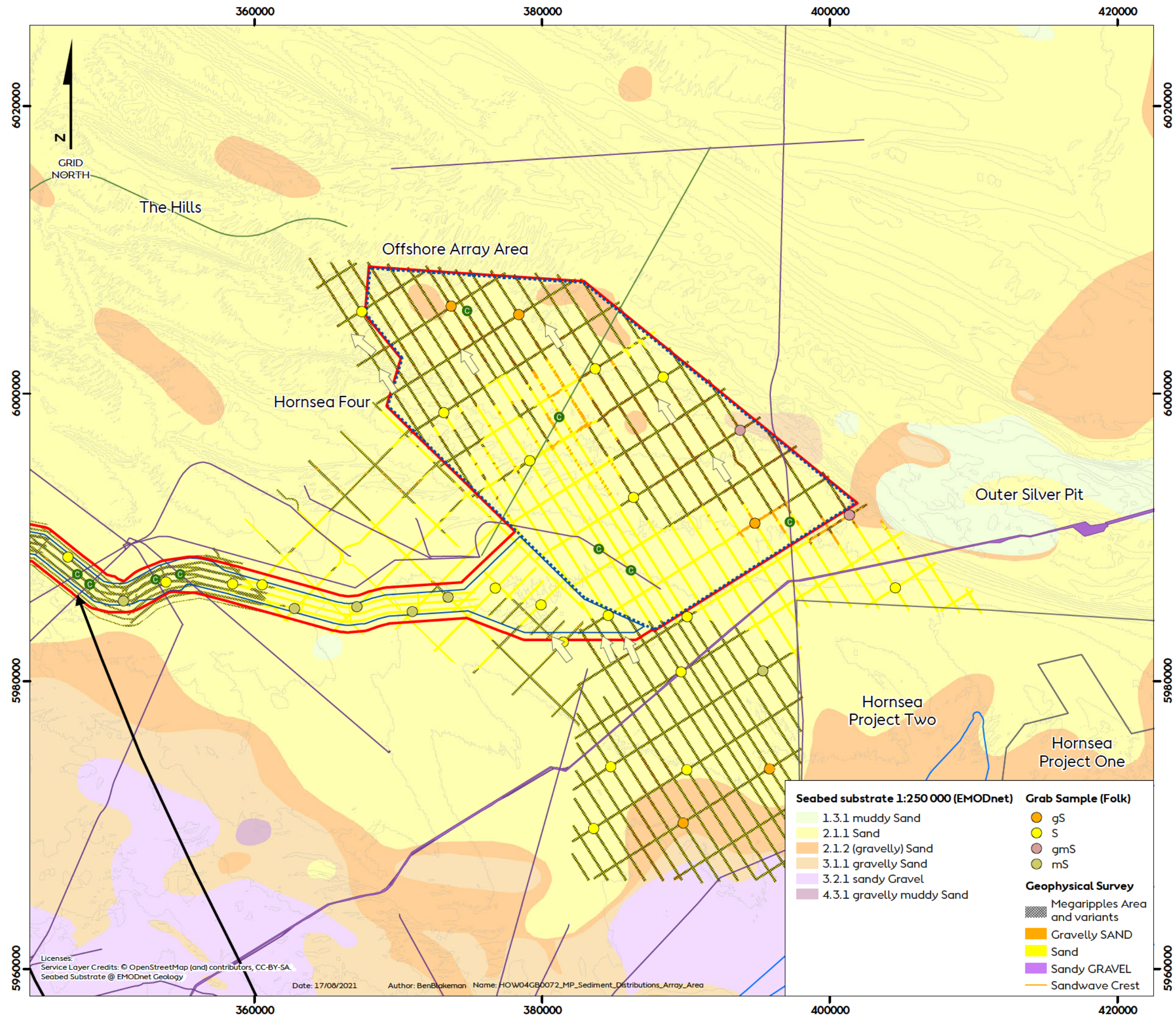
Figure 2 Sediment distributions across the offshore array study area
